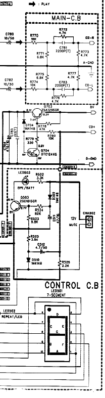
SCHEMATIC DIAGRAM (ULM-VERSION) MODEL NO. : ZCD-9 (AM/FM)
